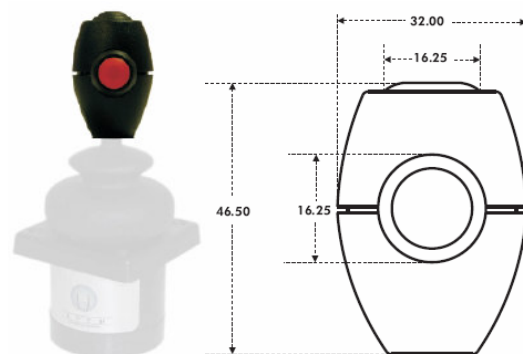
Handle X Multifunctional handle with 2 momentary IS series switches (one on top & one on the front)
