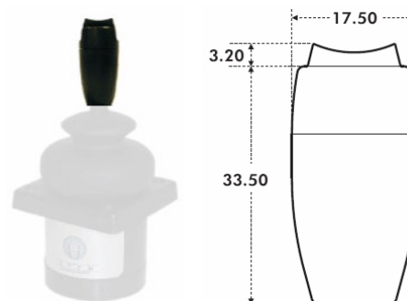
Handle AE Rocker switch handle with a Left & right rocking action TR series switch
