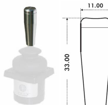
Handle AH A small modern-looking stainless steel handle with a polished finish
