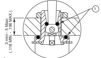
① O-rings
