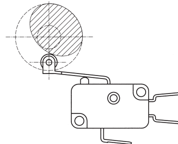
Long roller lever with continuous actuation
