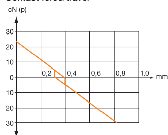
Contact force/travel
