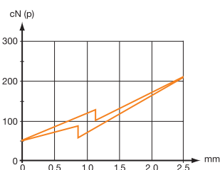
Actuating force/travel
