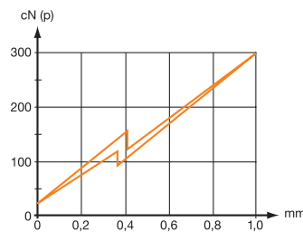
Actuating force/travel
