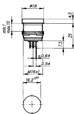
Ø 18, raised housing, Molex-style 3 pin
