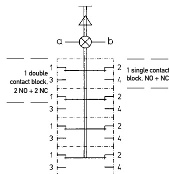
1 single contact block + 1 double contact block
