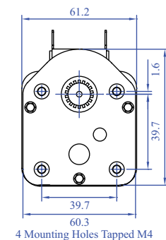
4 Mounting Holes Tapped M4
