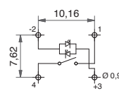
Bicolor - 2 LEDs
