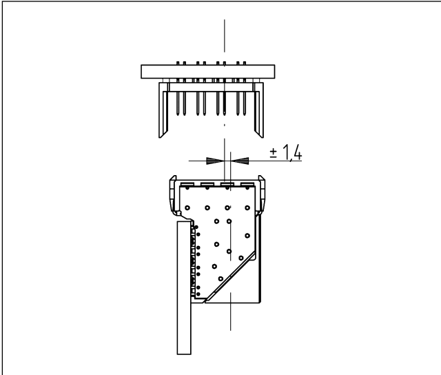
Transverse axis
