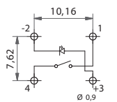
Single LED
