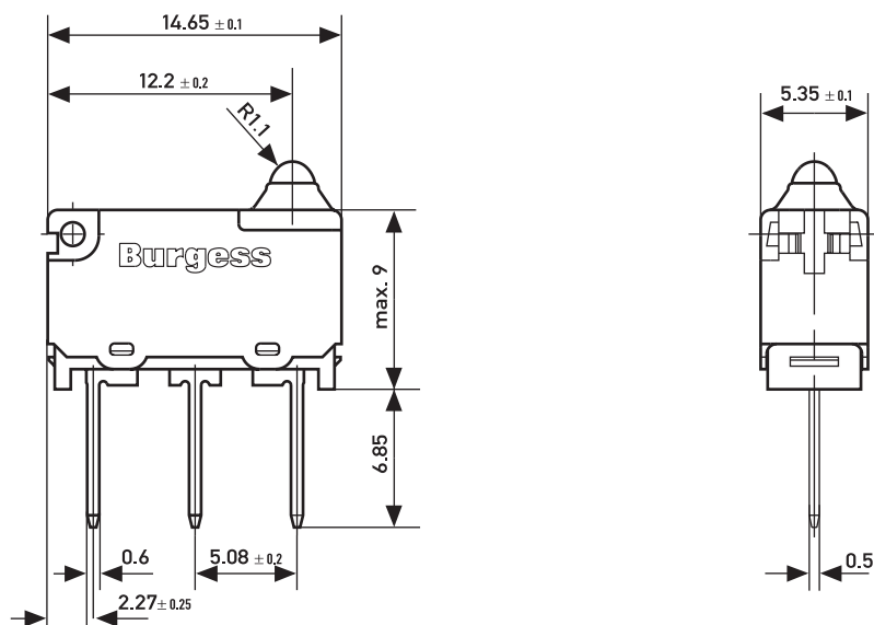
Dimensions L16T85
