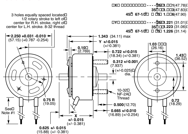
Double Shaft
