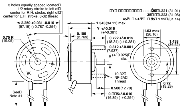
Double Shaft
