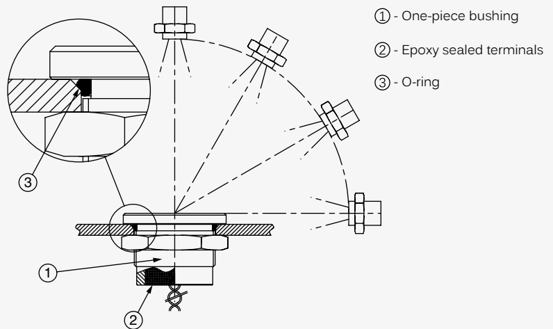
SEALING IP69K
