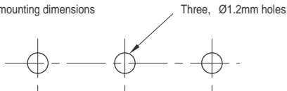
PCB mounting dimensions
