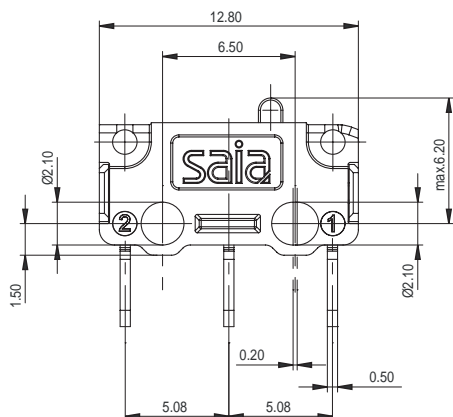
PCB mounting dimensions
