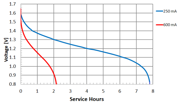
Constant Current
