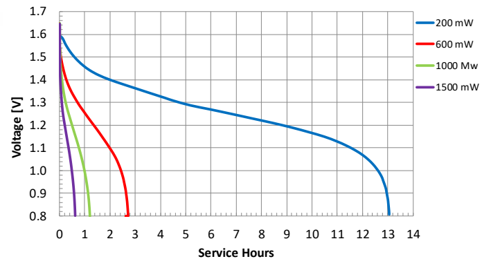
Constant Power
