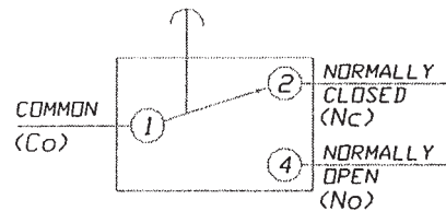
DIAGRAM OF CONNECTIONS
