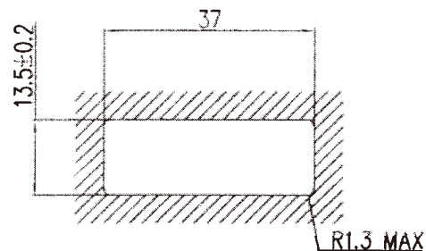
PANEL THICKNESS 1.0 – 2.5
